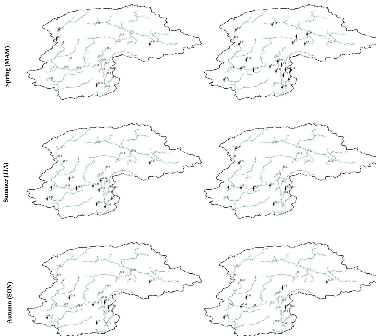
Figure 4: Spatial distribution of trends detected by Mann-Kendal and estimated by Sen's method in annual and seasonal maximum temperature showing change in °C decade -1 . (Upward and downward arrow shows positive and negative trends respectively, bold arrow shows significant at \alpha=0.1 )
