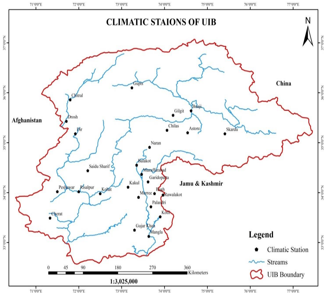
Fig 2: The (UIB) showing climatic stations, rivers and catchment area laying in Pakistan
