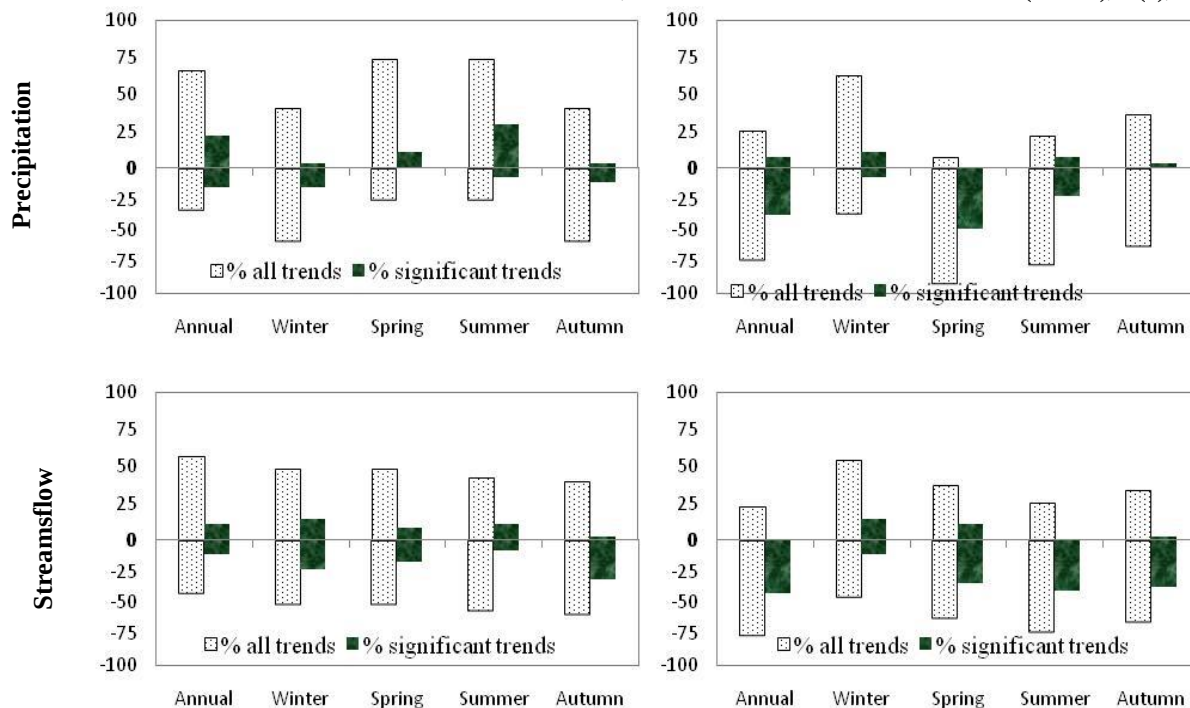
Figure 8: Percent number of stations with positive (upward) and negative (downward) trends in annual and seasonal time series for different periods and number of stations with significant trends by Mann-Kendall test at \alpha=0.1 .
