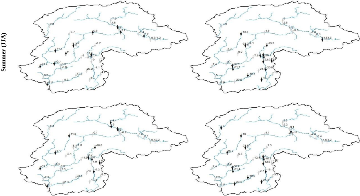
Figure 7: Spatial distribution of trends detected by Mann-Kendal and estimated by Sen’s method in annual and seasonal streamflows showing change in °C decade -1 . (Upward and downward arrow shows positive and negative trends respectively, bold arrow shows significant at \alpha=0.1 )
