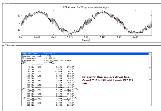
Figure 18: FFT analysis for Voltage wave form with D-STATCOM based on generalized technique.
