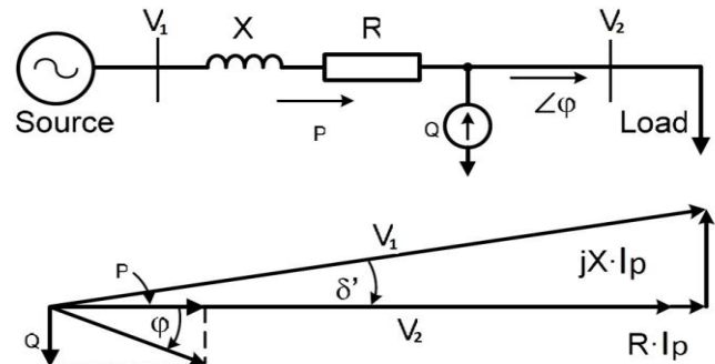
Figure 3: Shunt Compensation for power system.
