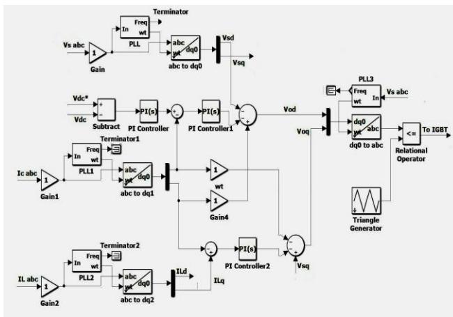
Figure 6: Park's Transformation Control Algorithm [11].
