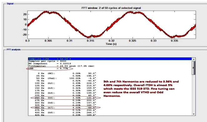
Figure 21: FFT analysis for Current wave form with D-STATCOM based on Park's Transformation technique.
