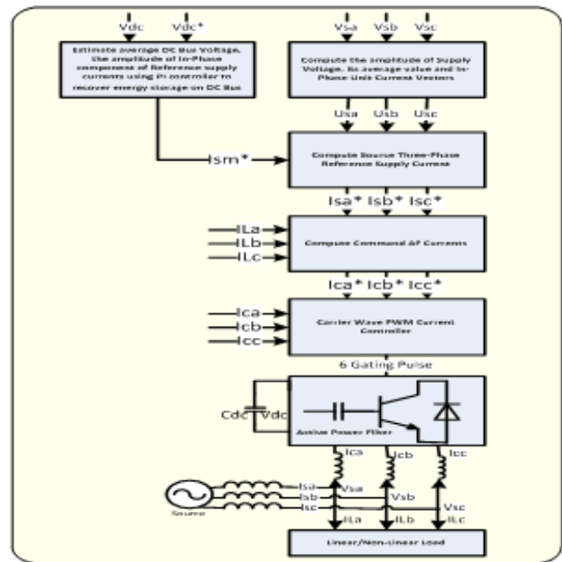
Figure 7: Generalized Control Algorithm [12]
