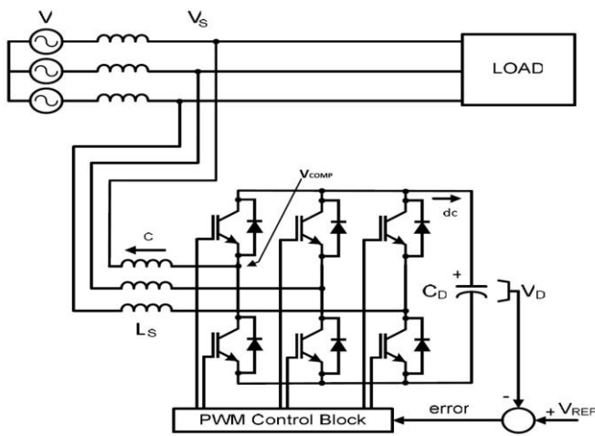
Figure 5: Connection of D-STATCOM [9].
