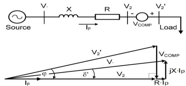
Figure 4: Series Compensation for power system.
