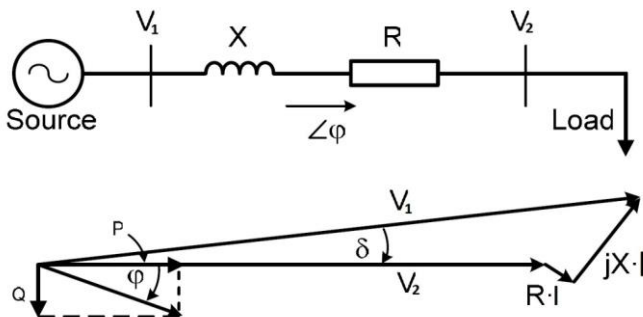
Figure 2: Power System without Compensation.
