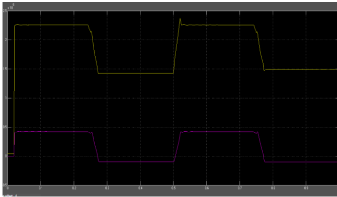
Figure 12: Reactive power drawn from grid during Microgrid Mode Switching without DSTATCOM.
