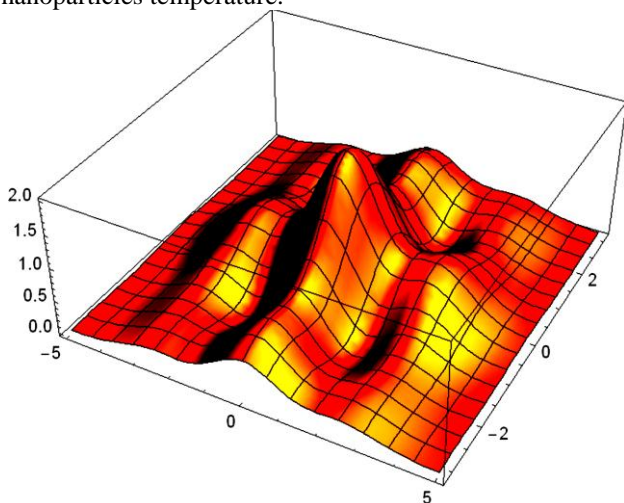
Figure 4: Maximum increase in temperature for core-shell Samarium nanospheres with various thicknesses of silica shell.
