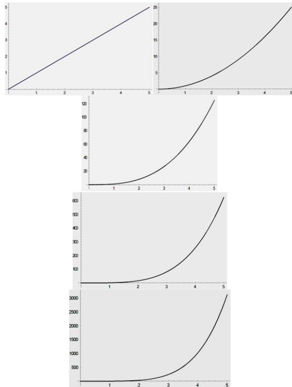
Figure 6: Extinction cross section area for Samarium nanorods with effective radius of 45 (nm) and various dimension ratios.
