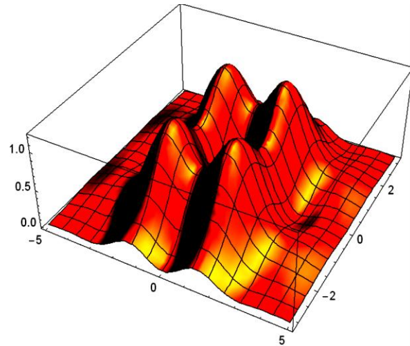
Figure 1: Maximum increase in temperature for Samarium nanospheres.
