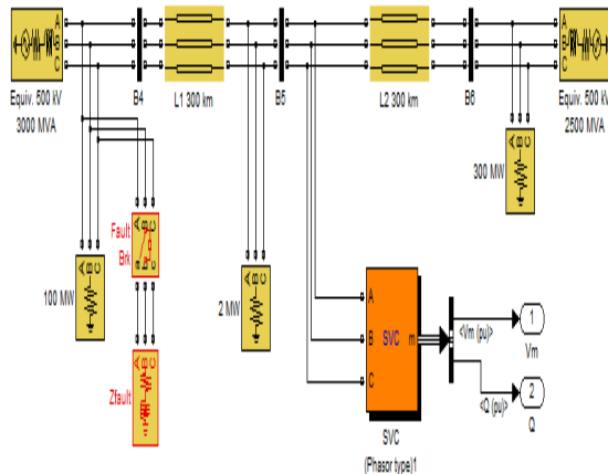
Figure 11- SVC model
