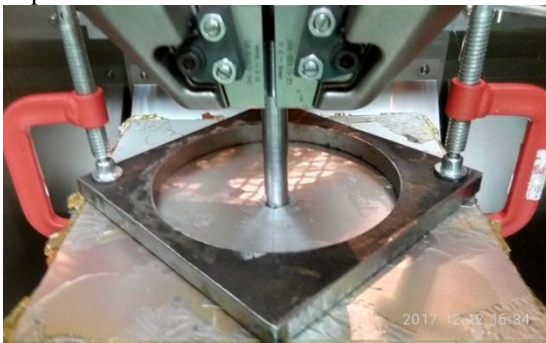
Fig (1): Quasi-static indentation specimen test setup
