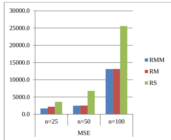
Fig.3. MSE of RMM, RM, RS for different sample sizes and 20% outliers
