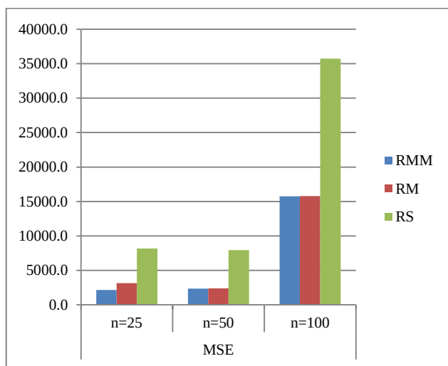
Fig.1. MSE of RMM, RM, RS for different sample sizes and 10% outliers
