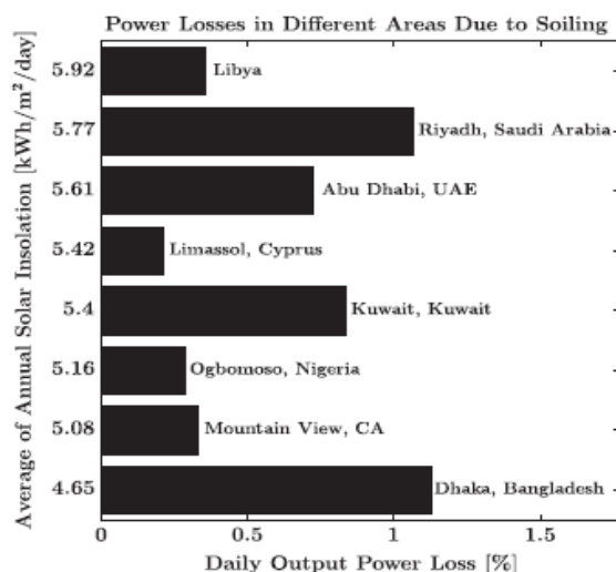
Figure 2: Daily Output Power Loss (%) [3]
