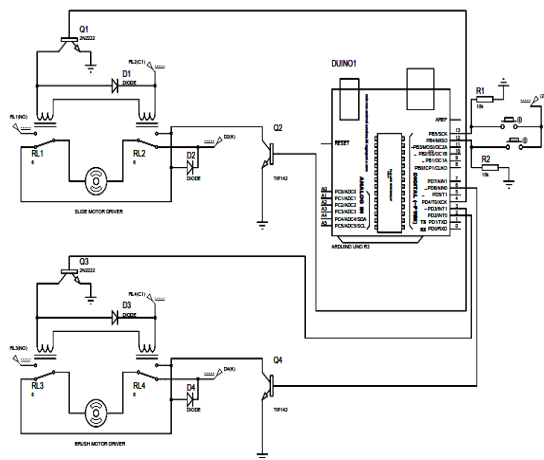
Figure 6: Complete Structure of Designed System
