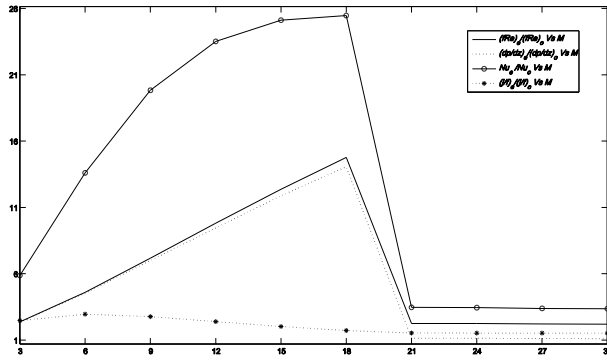
Fig. 5 Relative friction factor, Nusselt number and surface flow area goodness factor of optimum configurations plotted against the number.
